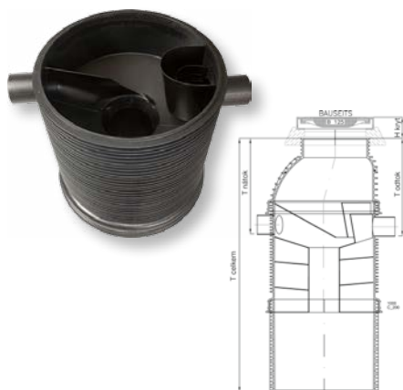
Certaro HDS Pro
